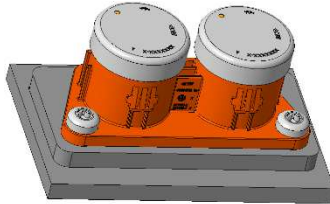
Figure 14: assemble housing assembly
