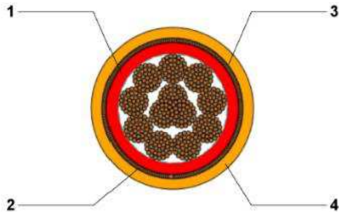
Figure 24: ISO HUBER SUHNER 70mm 2 Part No: 84100298
