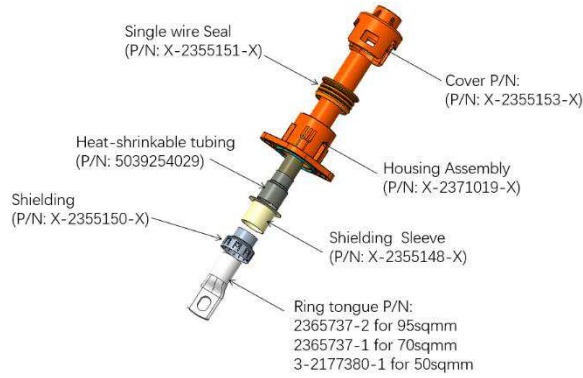
Figure 1: explosion view
