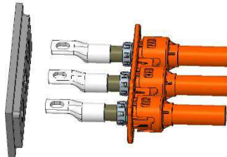
Figure 22: remove plug assembly
