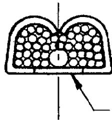
Cutoff tab centered with centerline of splice within .015 TIR.
