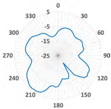
XZ-2.6GHz
