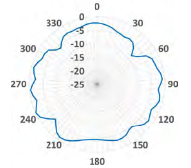
XY-5.3GHz
