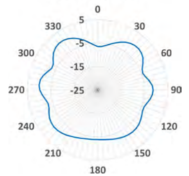
XY-2.6GHz
