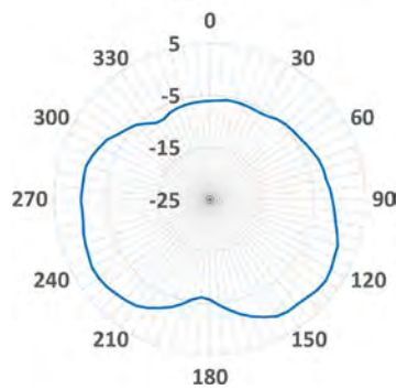
YZ-2.6GHz
