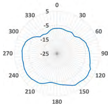
YZ-2.6GHz
