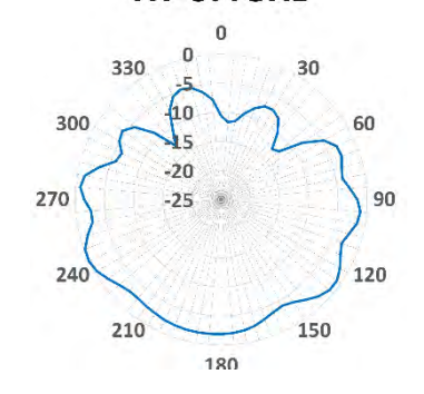
XY-3.4GHz
