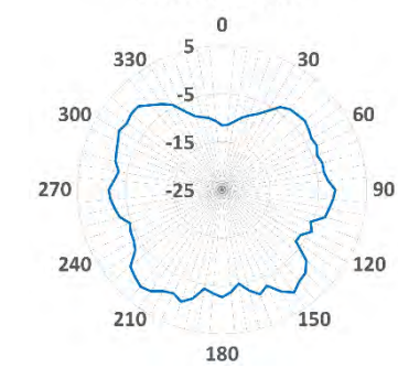
YZ-3.4GHz
