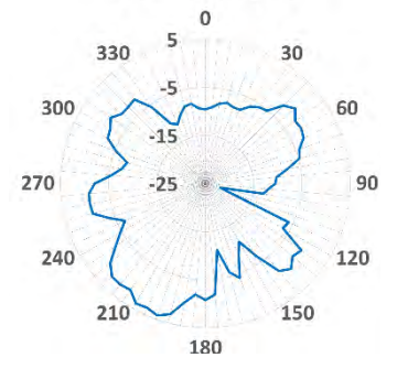
XZ-3.4GHz
