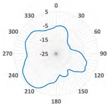
XZ-2.6GHz
