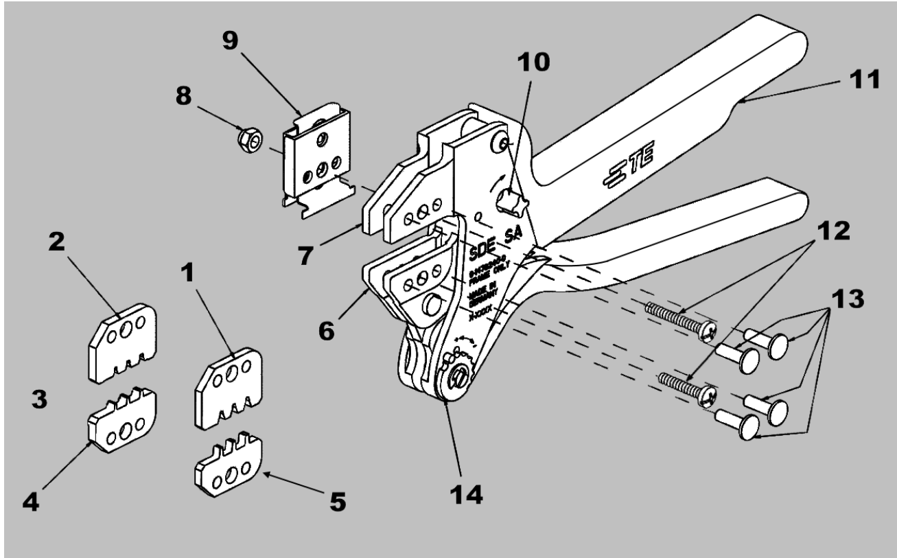
Figure 1: SDE-SA Commercial Hand Tool Assembly 2379968-1 with Die Assembly 2379968-2
