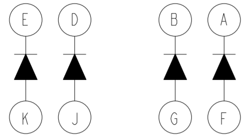
SCHEMATIC DIAGRAM (4) JANTX1N5552 DIODES
