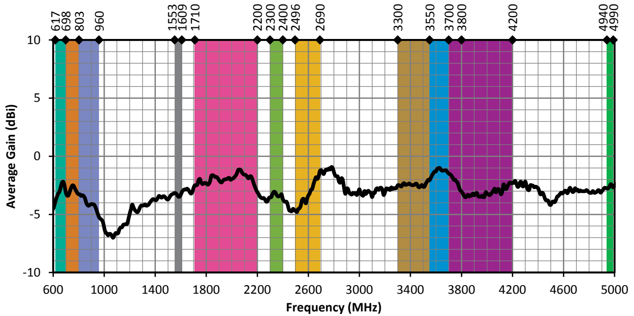
Figure 7. ANT-5GWWS5-SMA Antenna Average Gain, Straight
