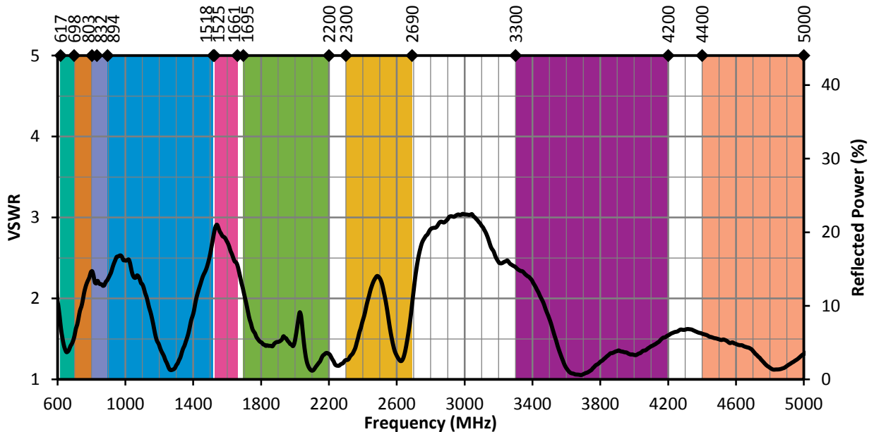
Figure 4. ANT-5GWWS5-SMA VSWR, Straight
