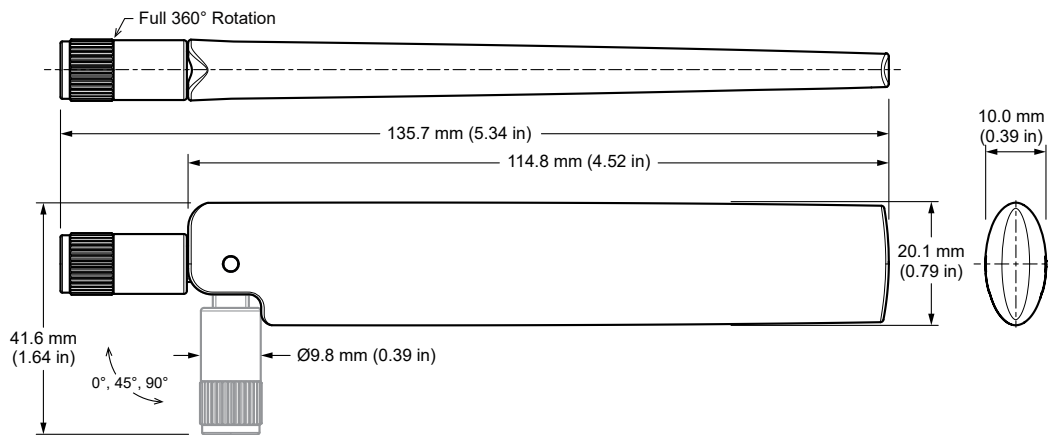
Figure 1. ANT-5GWWS5-SMA Antenna Dimensions
