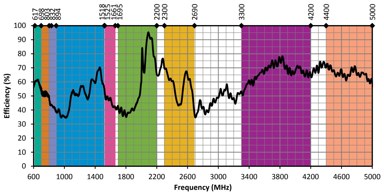
Figure 8. ANT-5GWWS5-SMA Antenna Efficiency, Straight
