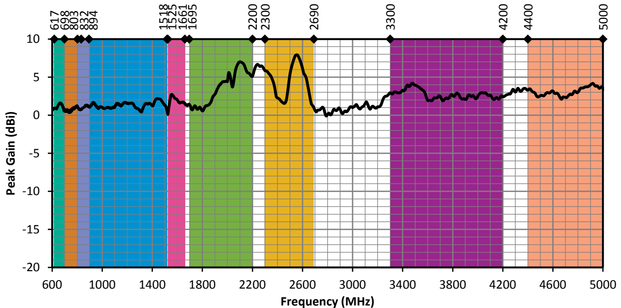
Figure 6. ANT-5GWWS5-SMA Peak Gain, Straight
