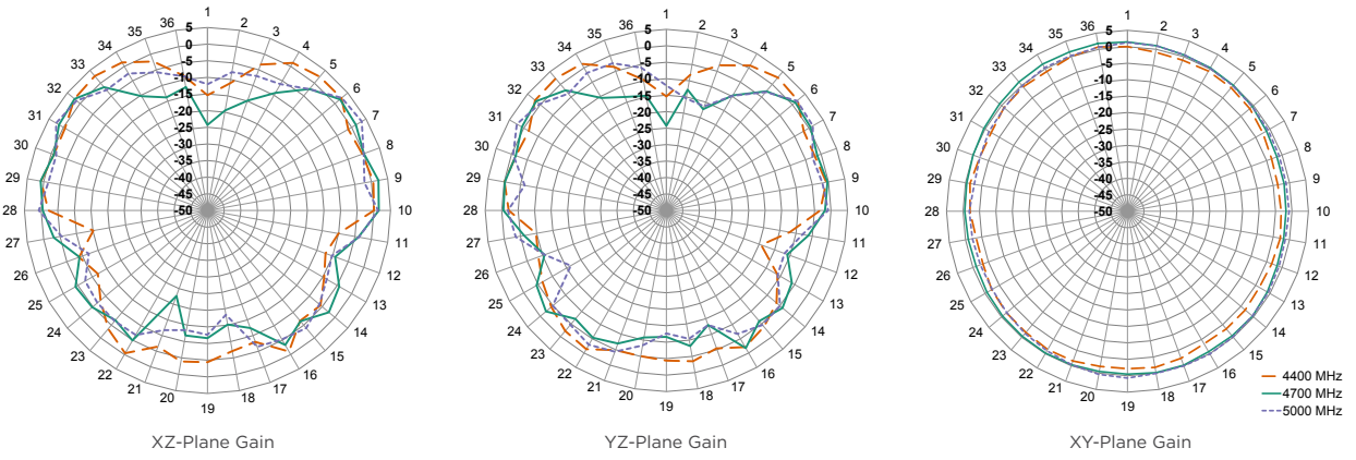
Figure 9. Radiation Patterns for ANT-5GWWS5-SMA, Straight
