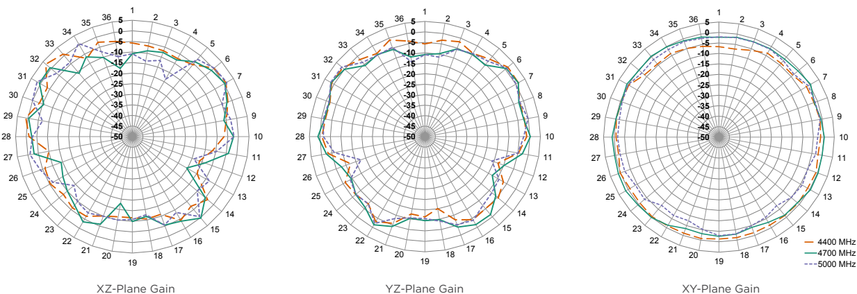
Figure 16. Radiation Patterns for ANT-5GWWS5-SMA, Edge-Bent
