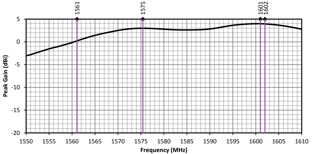
Figure 6. ANT-GNCP-TH25AL12 Peak Gain, L1 Bands
