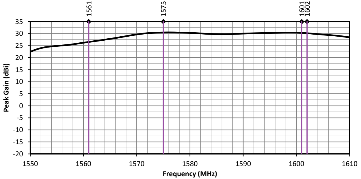
Figure 7. ANT-GNRM-L15A Series Antenna Peak Gain, L1 Band
