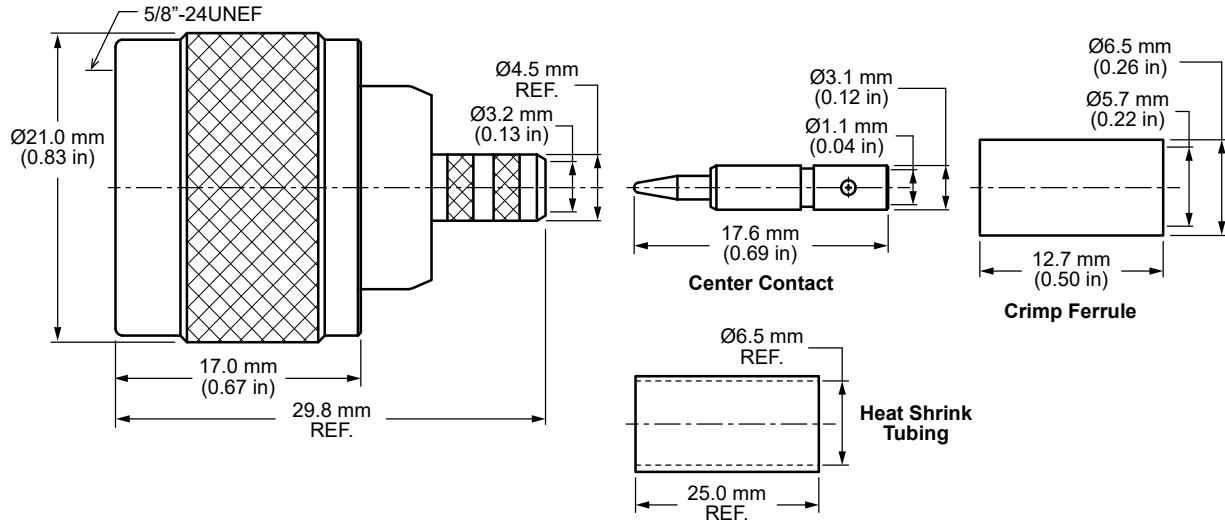
Figure 1: Product Dimensions for the CONN007-4-W Connector
