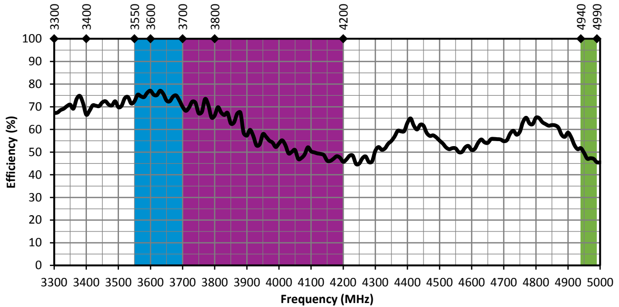
Figure 8. ANT-5GMWS1-SMA Antenna Efficiency, Straight
