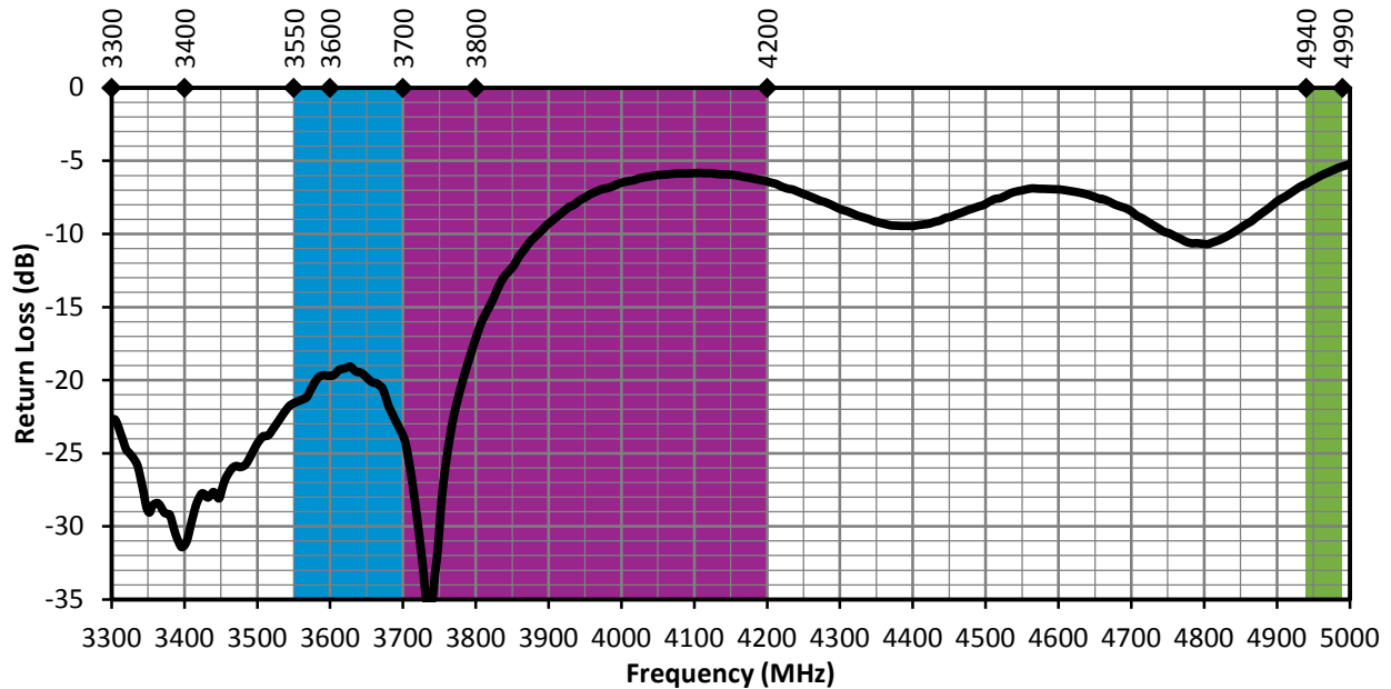
Figure 12. ANT-5GMWS1-SMA Return Loss, Edge-Bent
