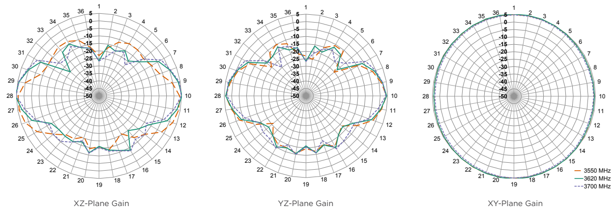
Figure 8. Radiation Patterns for the 5GMWS1, Straight
