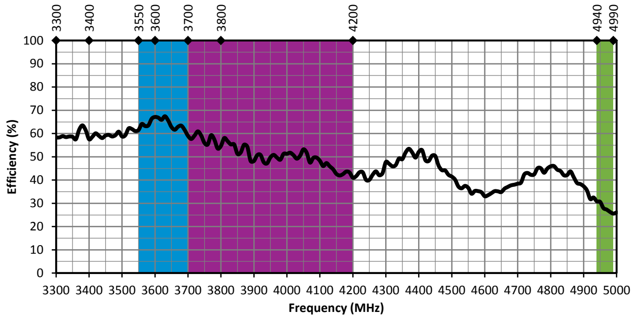
Figure 15. ANT-5GMWS1-SMA Antenna Efficiency, Edge-Bent
