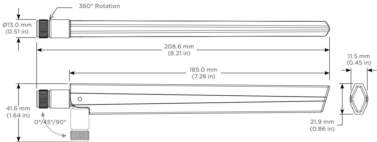
Figure 1: ANT-5GMWS1-NP Antenna Dimensions
