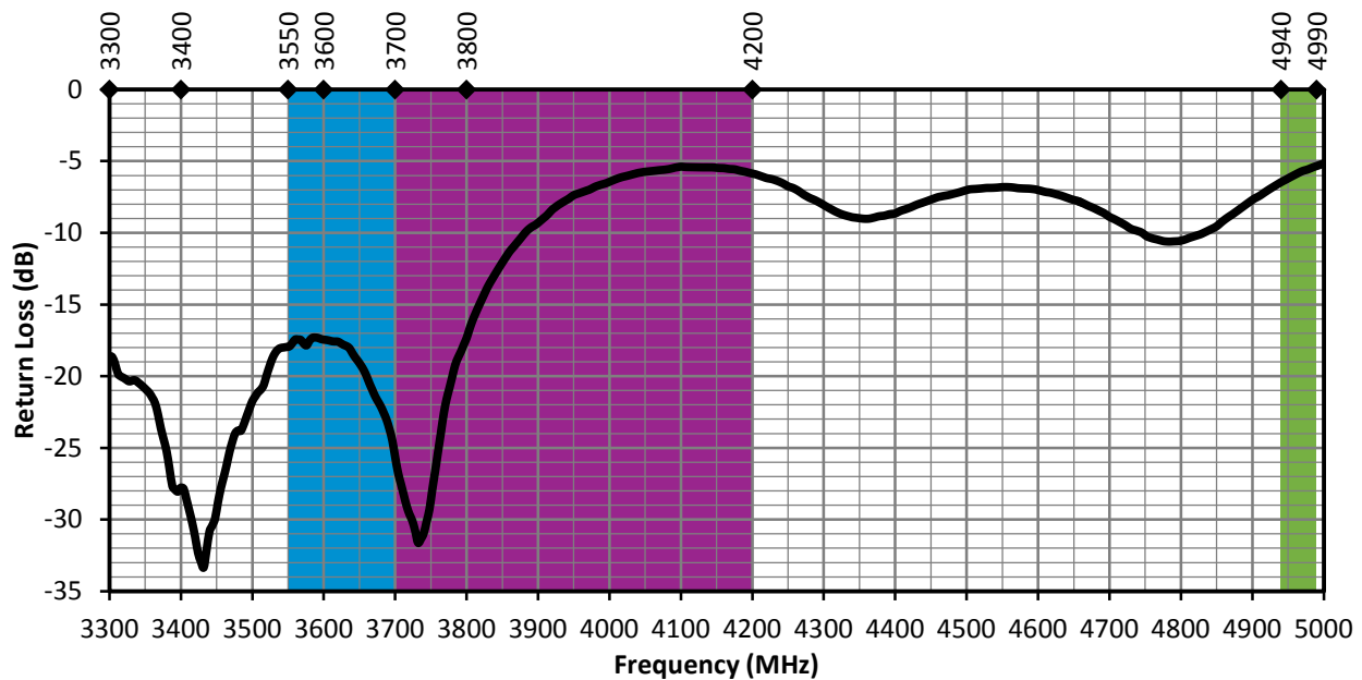
Figure 5. ANT-5GMWS1-SMA Return Loss, Straight
