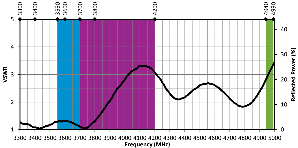
Figure 4. ANT-5GMWS1-SMA VSWR, Straight
