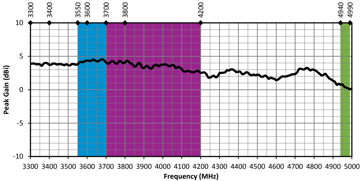
Figure 13. ANT-5GMWS1-SMA Peak Gain, Edge-Bent
