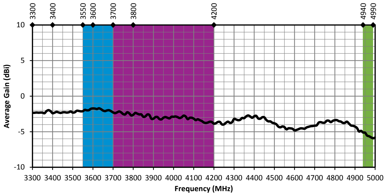
Figure 14. ANT-5GMWS1-SMA Series Antenna Average Gain, Edge-Bent
