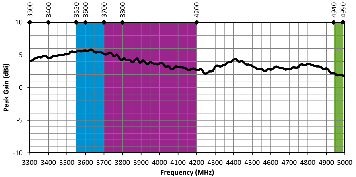
Figure 6. ANT-5GMWS1-SMA Peak Gain, Straight
