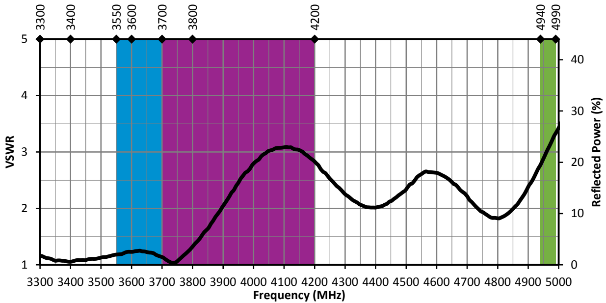
Figure 11. ANT-5GMWS1-SMA VSWR, Edge-Bent
