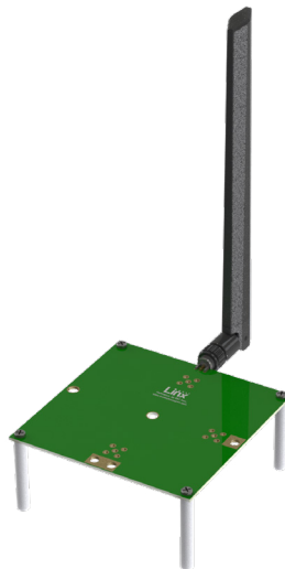
Figure 10. ANT-5GMWS1-SMA on Edge of Ground Plane, Bent 90 Degrees (Edge-Bent)
