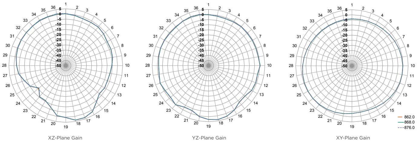
Figure 8. ANT-868-CW-RCL Radiation Patterns
