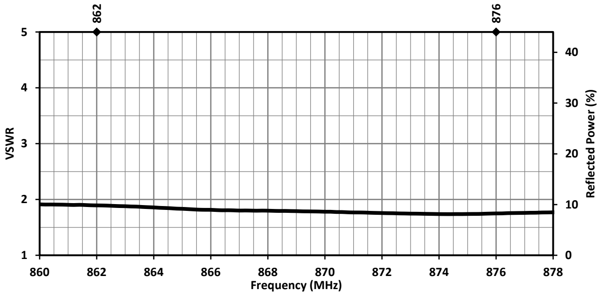
Figure 3. ANT-868-CW-RCL VSWR
