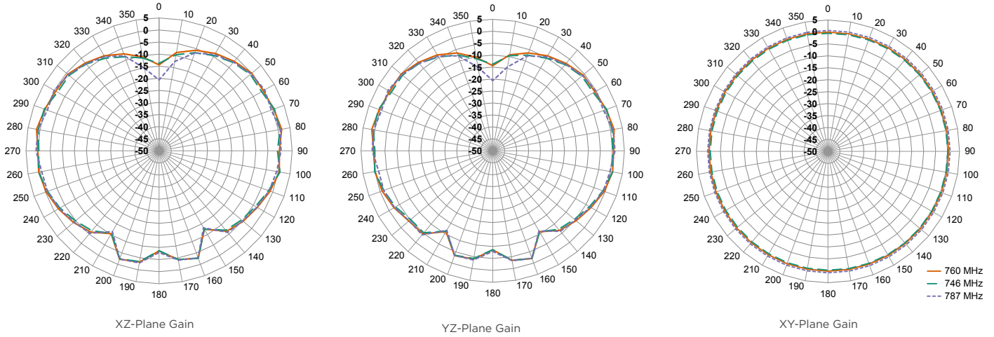
Figure 9: Radiation Patterns for PW LTE Band 13 Antenna
