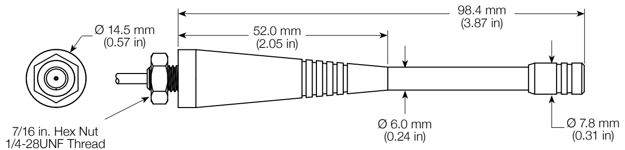
Figure 7: PW LTE Band 13 Antenna Dimensions
