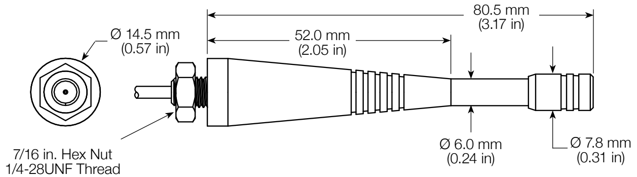
Figure 7: PW LTE Band 8 Antenna Dimensions
