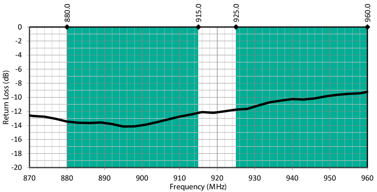
Figure 3: PW LTE Band 8 Antenna Return Loss with Band 8 Uplink/Downlink Highlights
