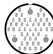
61-949 46 Size 20 Contacts 3 Size 8 Contacts
