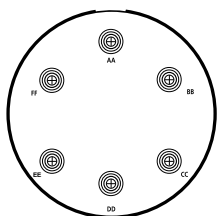
28-06 6 Size K6 Contacts *
