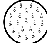
22-21 21 Size 16 Contacts
