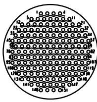
23-23 151 Size 23 Contacts
