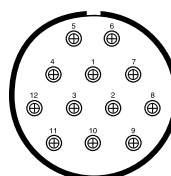
61-21 12 Size 8 Contacts *
