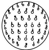
25-43 20 Size 16 Contacts 23 Size 20 Contacts
