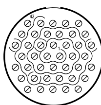
28-42 42 Size 16 Contacts *
