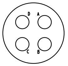
21-76 4 Size 8 Twinax Contacts
