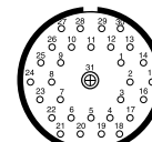
37-13 30 Size 20 Contacts 1 Size 8 Contact
