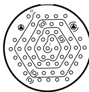
24-57 55 Size 20 Contacts 2 Size 12 Contacts *
