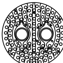
25-09 2 Size 8 Twinax Contacts 97 Size 22D Contacts
