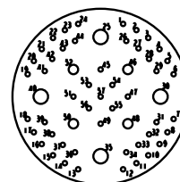
23-63 4 Size 12 Contacts 4 Size 16 Contacts 49 Size 22D Contacts
