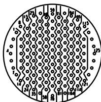
25-01* 128 Size 22D Contacts
