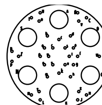
25-17 6 Size 8 Twinax Contacts 36 Size 22D Contacts
