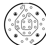
20-28 24 Size 20 Contacts 4 Size 12 Contacts
