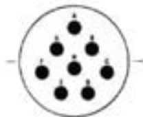
16-8* 8 Size 16 Contacts
