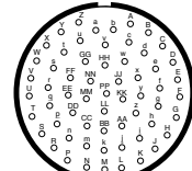
24-61 61 Size 20 Contacts
