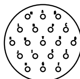
15-19 19 Size 20 Contacts
