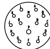
15-15 14 Size 20 Contacts
