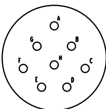
17-08 8 Size 16 Contacts
