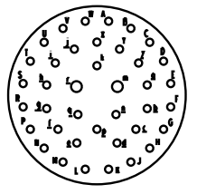
21-39 2 Size 16 Contacts 37 Size 20 Contacts
