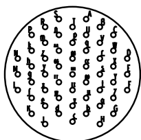
23-53 53 Size 20 Contacts
