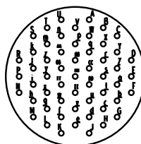
23-55 55 Size 20 Contacts
