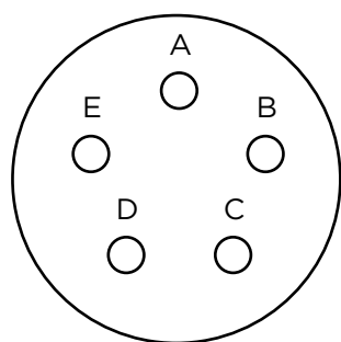
14-5 5 Size 16 Contacts
