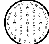
22-41 27 Size 20 Contacts 14 Size 16 Contacts
