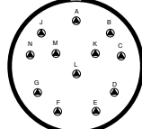
22-12 12 Size 12 Contacts
