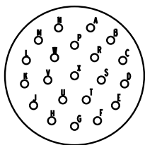
23-21 21 Size 16 Contacts
