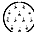
37-3 12 Size 12 Contacts *
