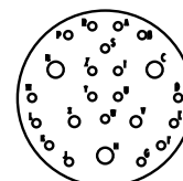
15-A23 4 Size 16 Coax Contacts 3 Size 20 Contacts 19 Size 22D Contacts
