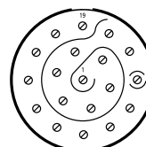
22-19 19 Size 16 Contacts
