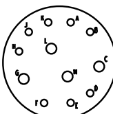
15-97 4 Size 12 Contacts 8 Size 20 Contacts
