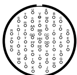
22-55 55 Size 20 Contacts
