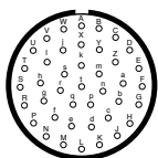
20-41 41 Size 20 Contacts
