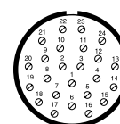
37-924 24 Size 16 Contacts *
