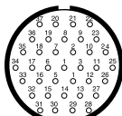
37-0 37 Size 20 Contacts *
