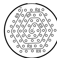
24-61 61 Size 20 Contacts
