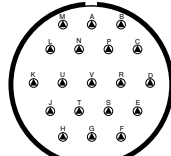
24-19 19 Size 12 Contacts
