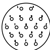
15-18 18 Size 20 Contacts
