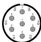
37-27 6 Size 20 Contacts 7 Size 8 Contacts *
