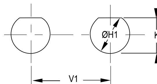
Jam Nut Receptacle (Type 24)
