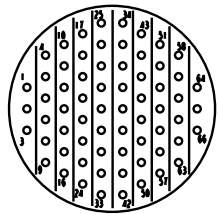
19-35 66 Size 22D Contacts
