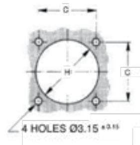
Panel Boring
