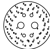
25-47 2 Size 8 Coax Contacts 4 Size 12 Contacts 40 Size 20 Contacts
