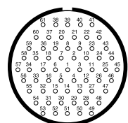
61-0 61 Size 20 Contact *
