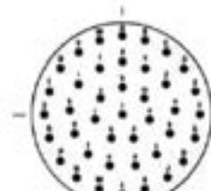
20-41 41 Size 20 Contacts
