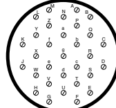
24-31 31 Size 16 Contacts
