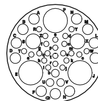
23-41 3 Size 8 Contacts 3 Size 12 Contacts 11 Size 16 Contacts 3 Size 20 Contacts 22 Size 22D Contacts
