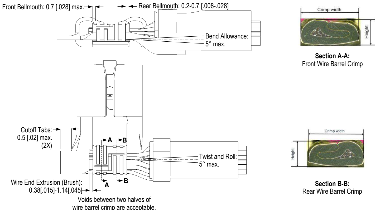
Figure 3A – Right-Hand 2D Flags PNs 2238171-3 and 2238172-3.
