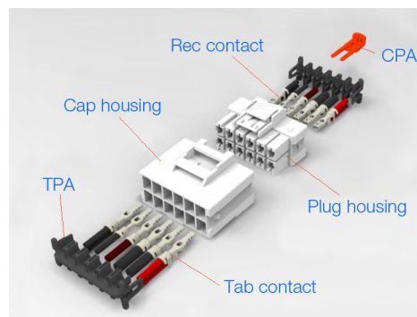
Figure 1. Product design components of the POWER TRIPLE LOCK connector. (2 rows as shown, single row and triple rows excluded here)
